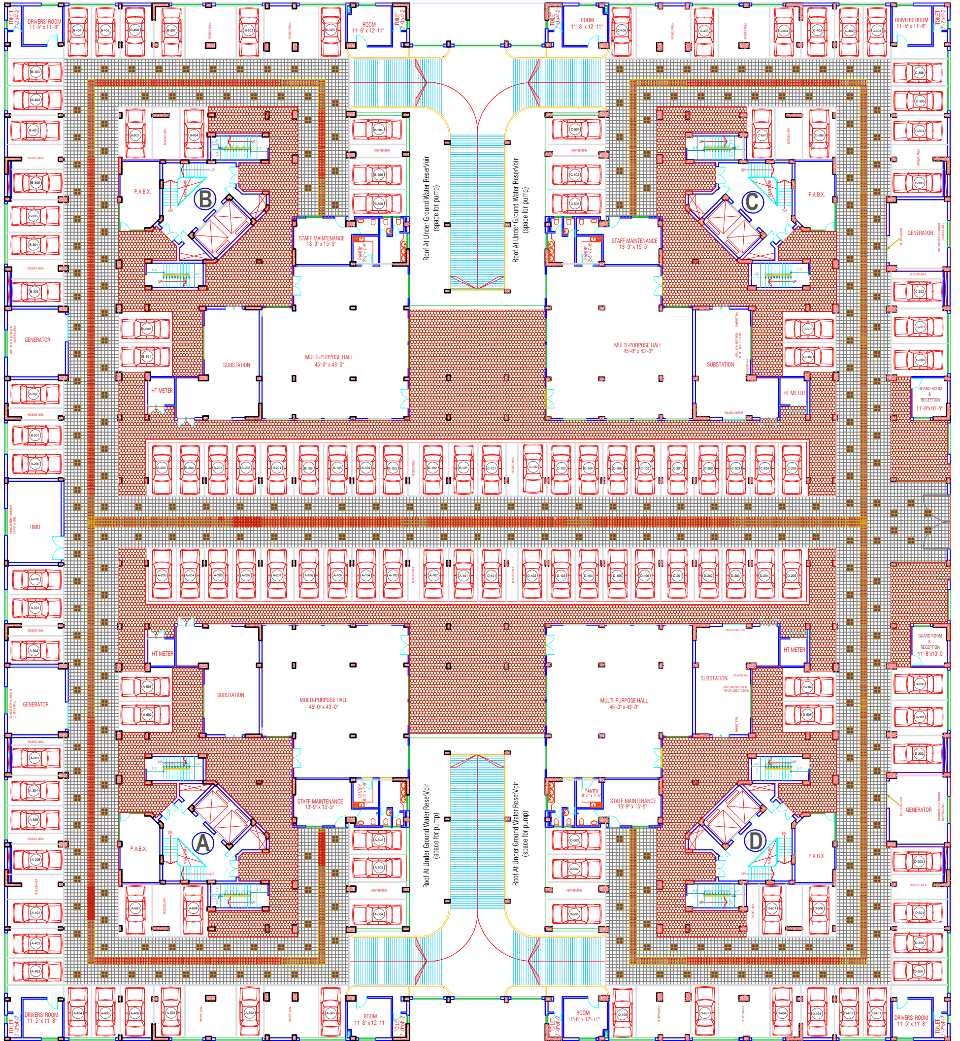
GROUND FLOOR PLAN (4-Bldg. Cluster) NOT TO SCALE
