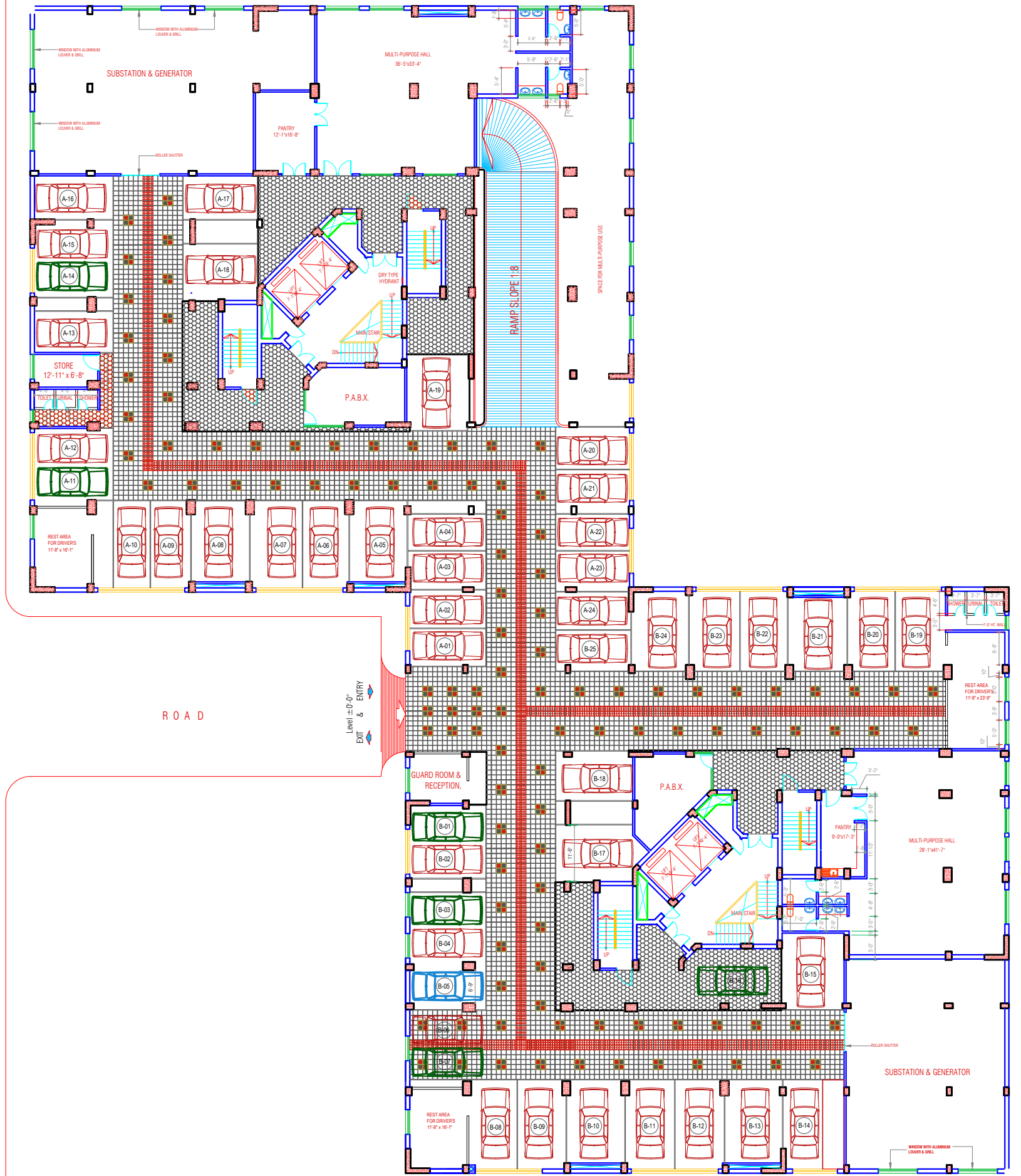
GROUND FLOOR PLAN (Bldg.-12A, 12F, 13A, 13B ) NOT TO SCALE
