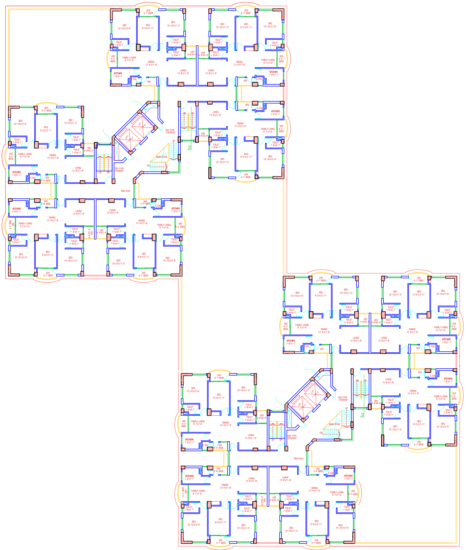
TYPICAL FLOOR PLAN (Bldg.-12A, 12F, 13A, 13B) NOT TO SCALE
