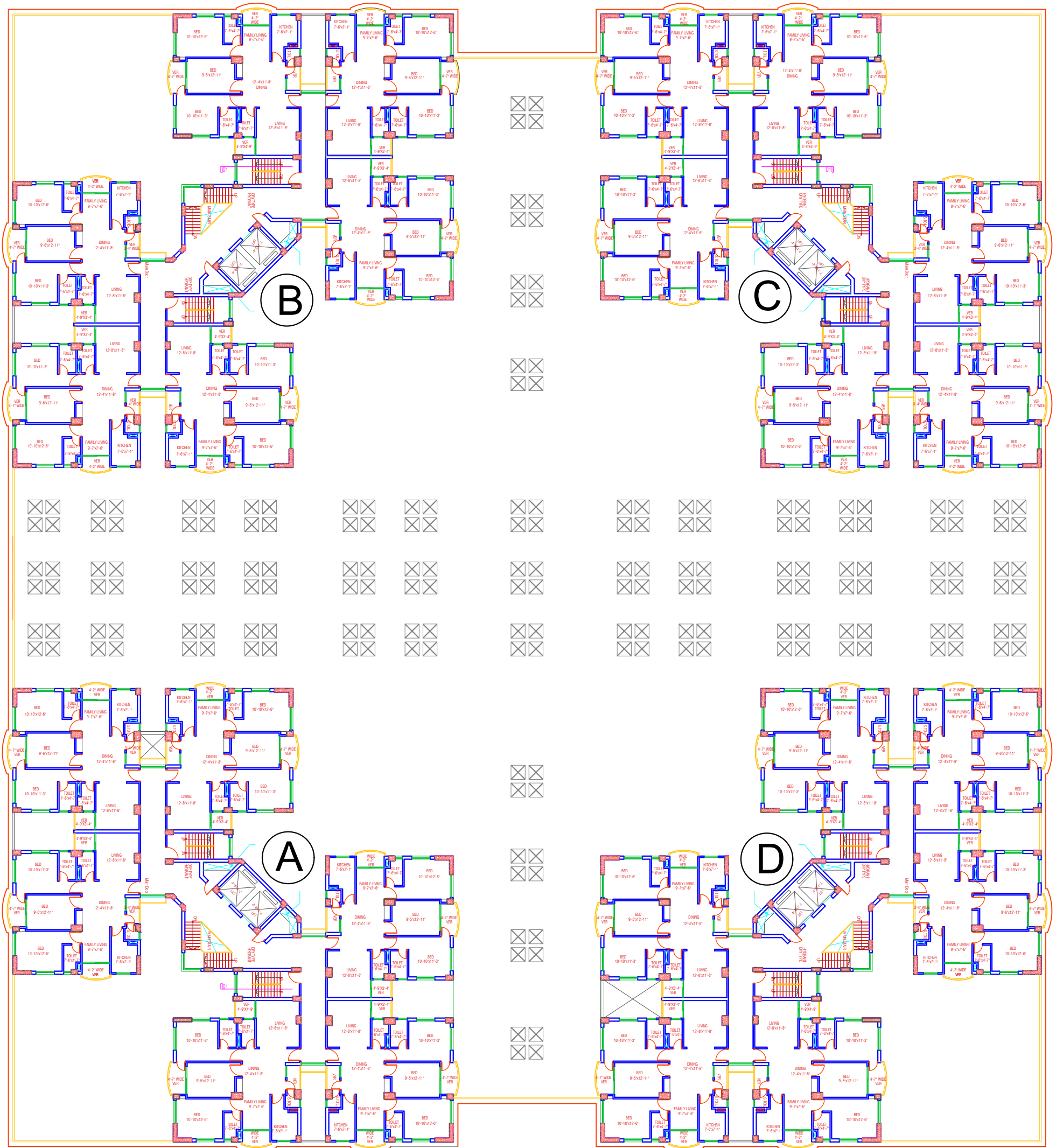
TYPICAL FLOOR PLAN NOT TO SCALE
